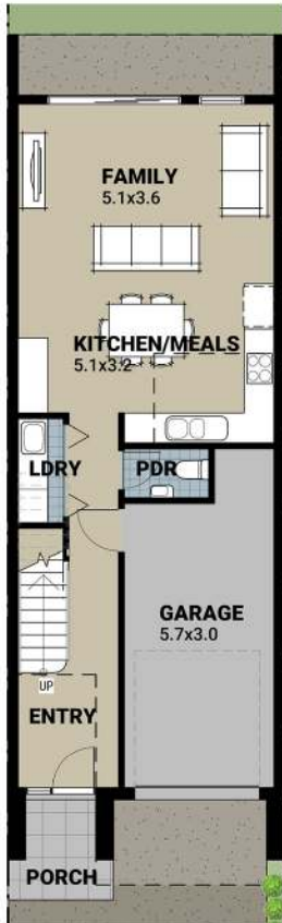
LOWER FLOOR PLAN
